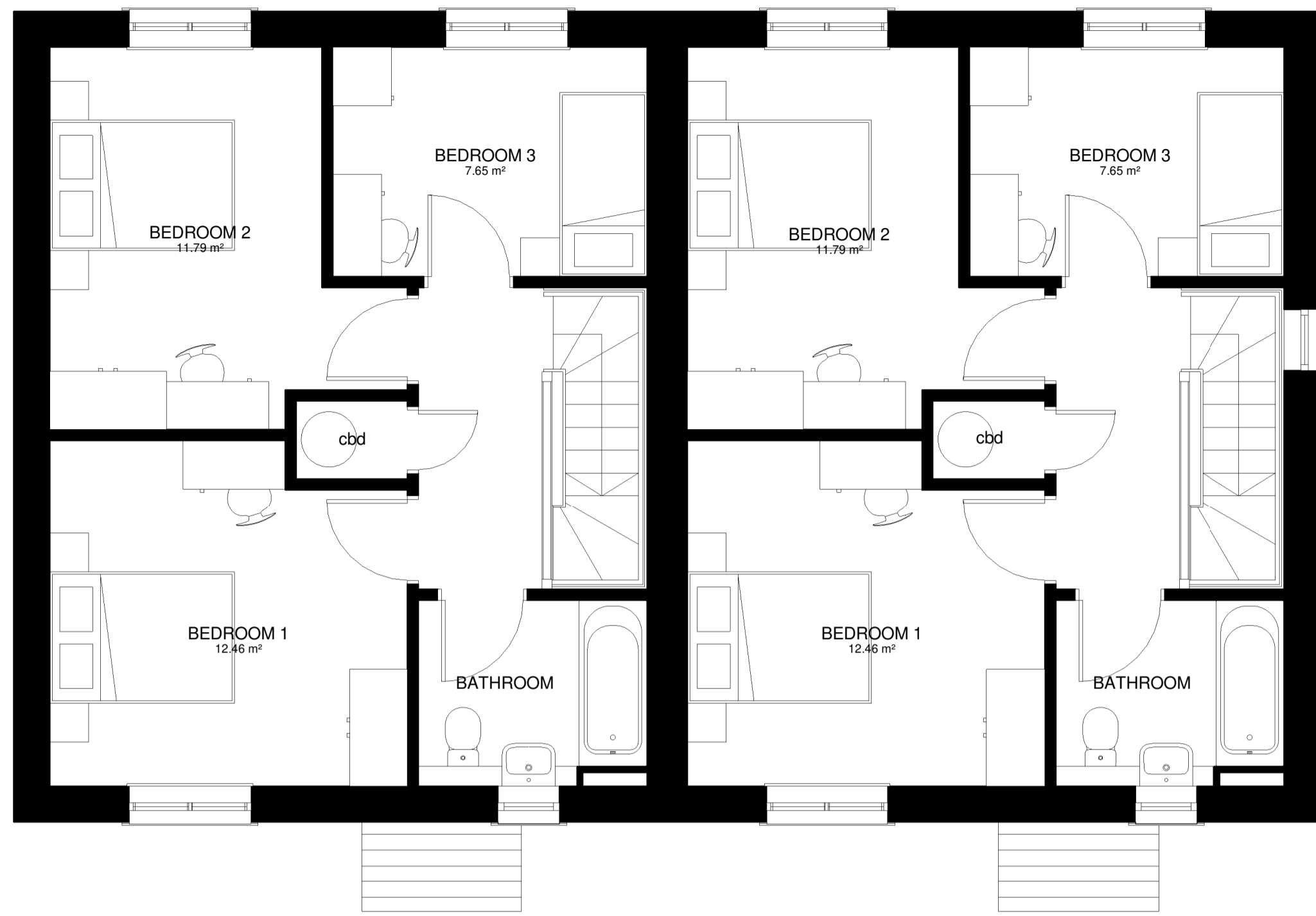
FIRST FLOOR layout 1 : 50
