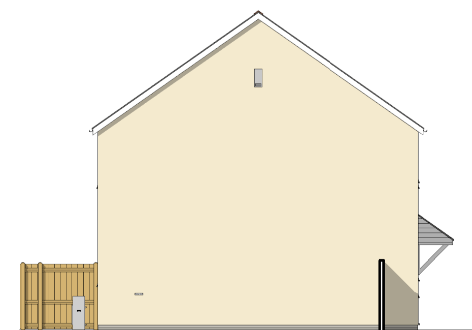
SOUTH EAST elevation 1 : 100
