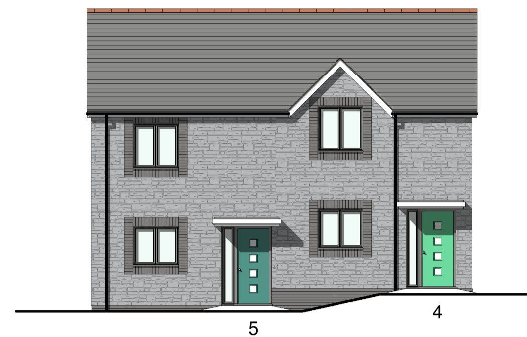
SOUTH elevation 1 : 100
