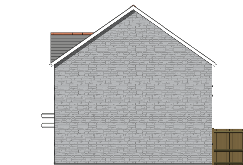
EAST elevation 1 : 100
