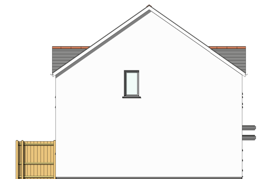
EAST elevation 1 : 100
