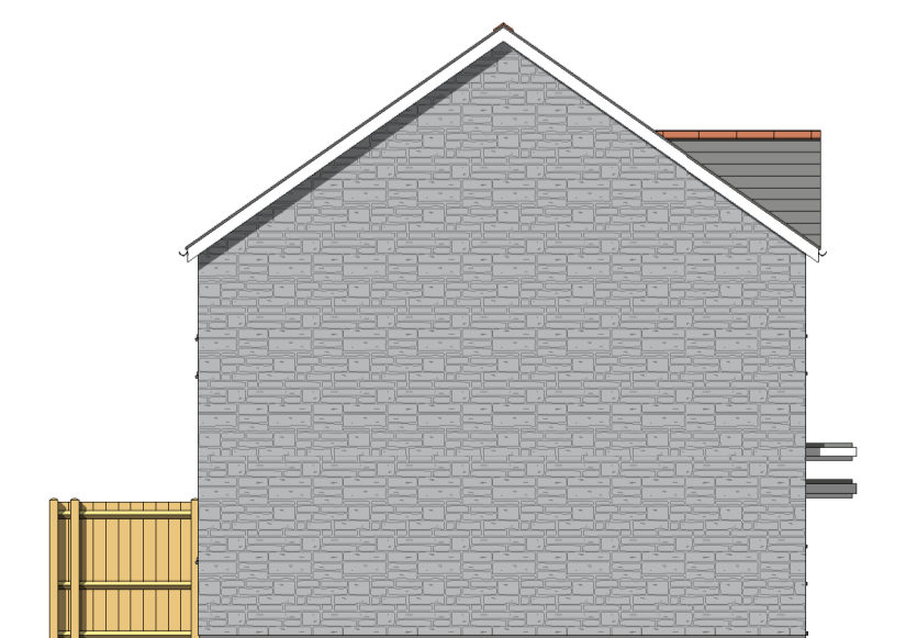
EAST elevation 1 : 100
