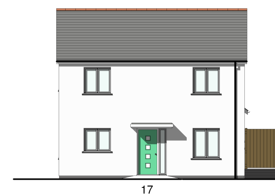
SOUTH WEST elevation 1 : 100
