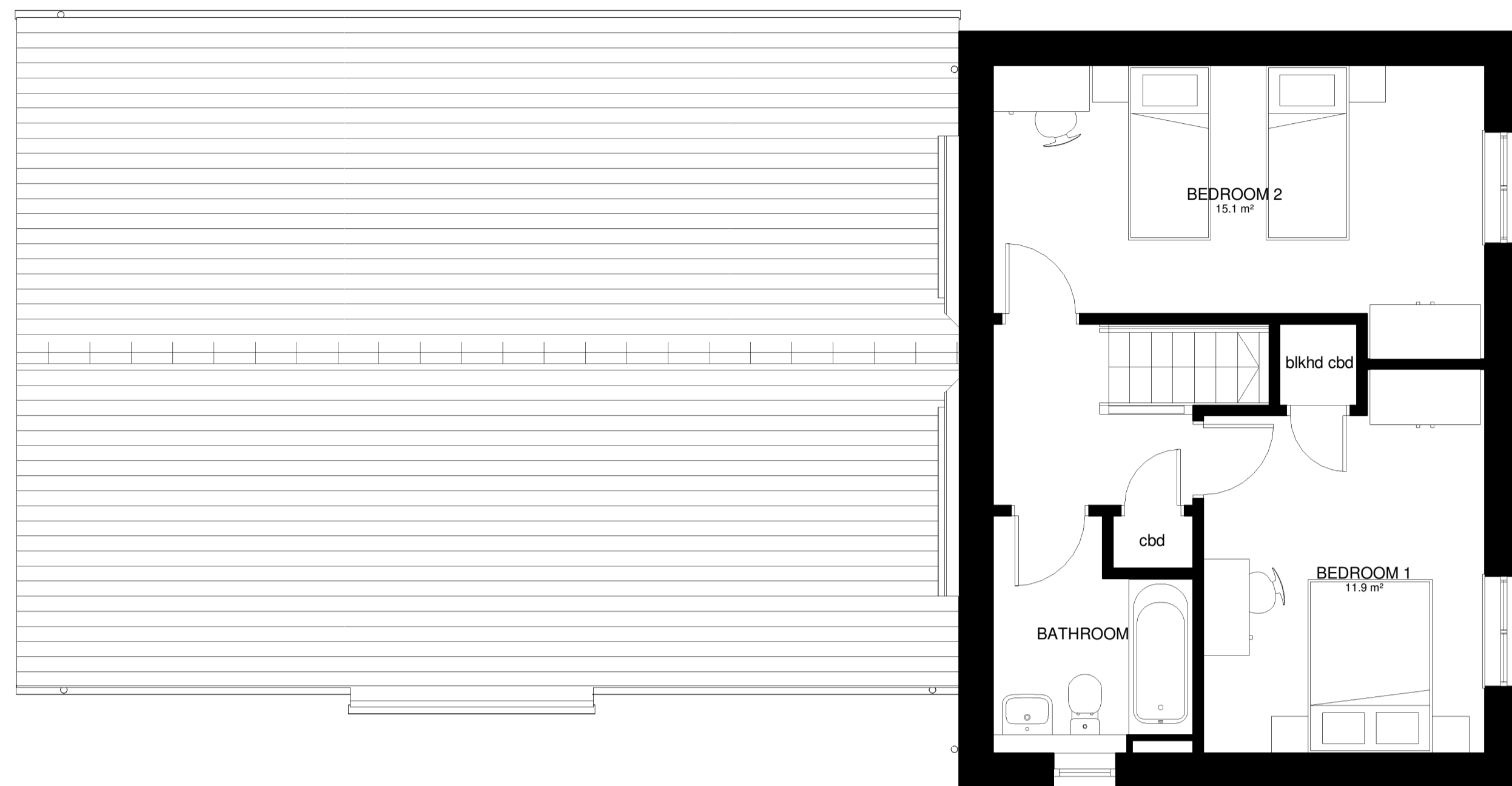
FIRST FLOOR layout 1 : 50
